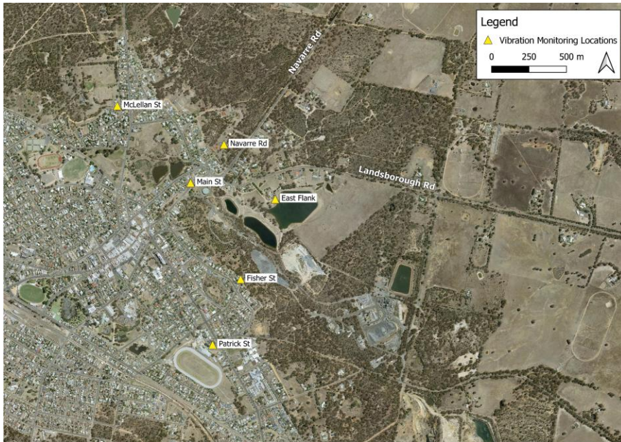
Figure 21 - SGM vibration monitoring locations
