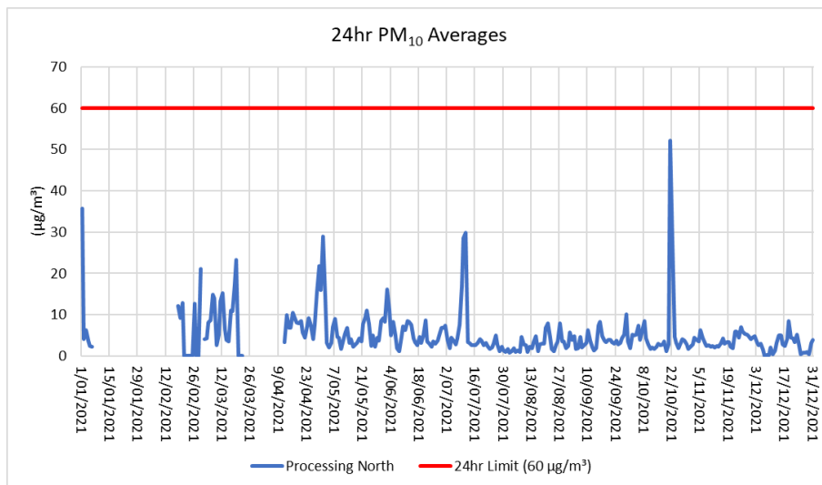
Figure 13 – Processing North PM 10 Results for 2021
