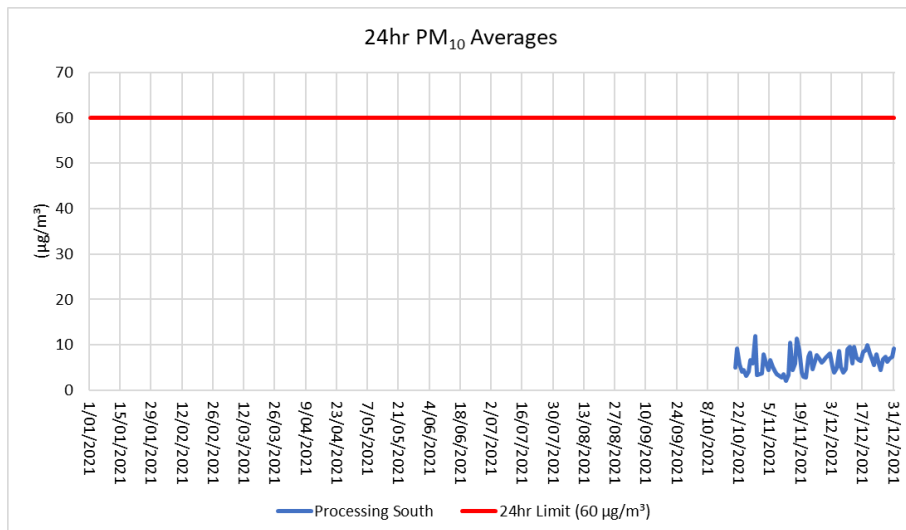
Figure 14 – Processing South PM 10 Results for 2021
